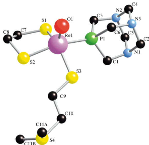
Figure 1. The molecular structure of [ReO( \kappa^2 -edt)( \kappa^1 -edtMe)(PTA)]. The methyl group at S 4 was disordered; the structure was refined at 50% occupancy of the two sites. Selected bond lengths [pm] and angles [°] are: Re–O 170.0(5), Re–S3 230.54(17), Re–P 242.25(18), S4–C10 181.0(9), S4–C11A 175.6(17), S4–C11B 184.0(4); O–Re–S3 110.68(19), O–Re–P 97.3(2), S2–Re–P 153.94(6), S1–Re–S3 133.58(7), C10–S4–C11A 102.7(7), C10–S4–C11B 104.3(17), C11A–S4–C11B 133.1(14). The structure was drawn with the CrystalMaker program. [13]
